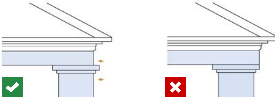
Porch Column to Beam Detail
