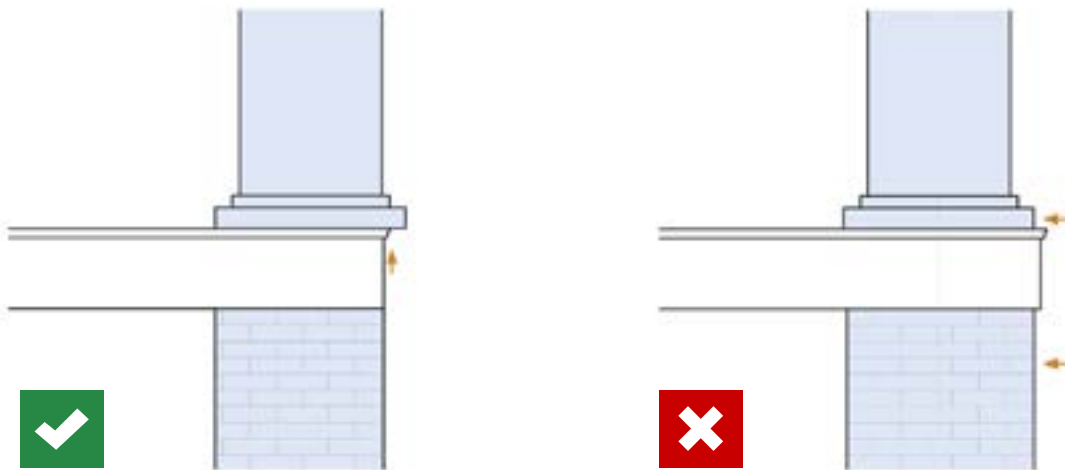
Porch Column to Floor Detail
